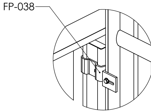
DETAIL C SCALE 1 : 5 Top post attachment
