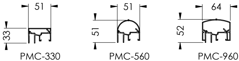
HANDRAILS
